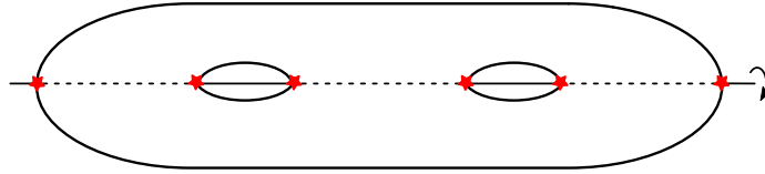
Figure 7.6.: We sketch the hyperelliptic involution of the closed surface of genus two. We highlight the 6 fixed points.
